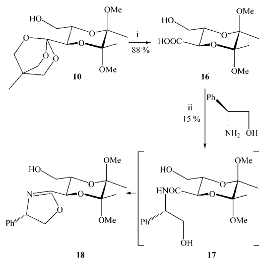
Scheme 3. Reagents and conditions: i) 1 M HCl, pH 1, 0 °C, 30 min, then 1 M LiOH, pH 11, reflux; ii) amino alcohol, decalin, reflux
