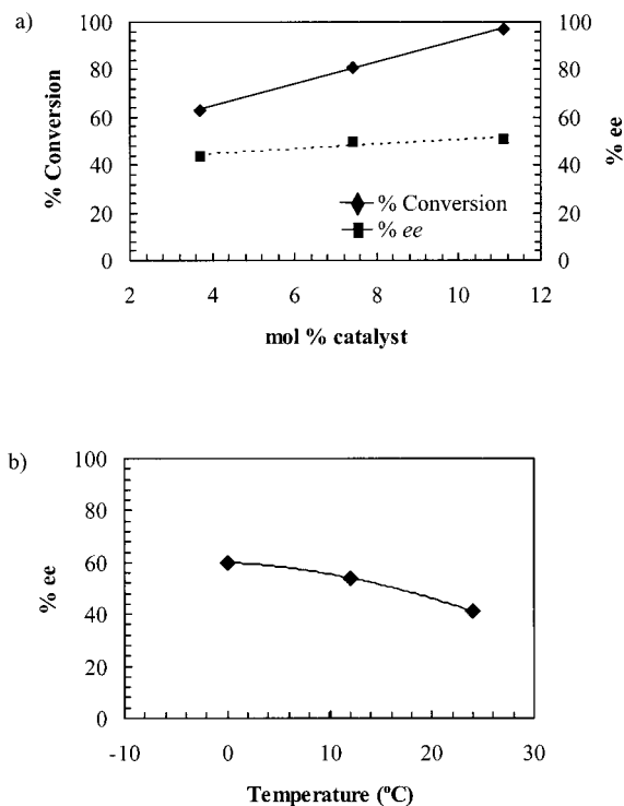
Figure 1. Variation of the ee as a function of the reaction conditions in the addition of diethylzinc to benzaldehyde catalyzed by 6a : a) the effect of the catalyst concentration on ee and on conversion after 24 h; b) the effect of temperature observed after 24 h. [26]
