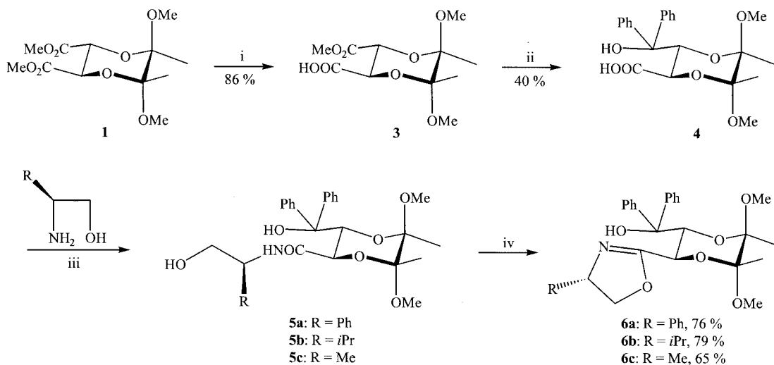
Scheme 1. Reagents and conditions: i) 1.2 equiv. KOH, MeOH, reflux; ii) 3 equiv. PhMgBr, THF, reflux; iii) amino alcohol, xylene, reflux; iv) p TsCl, Et 3 N, CH 2 Cl 2 , reflux
