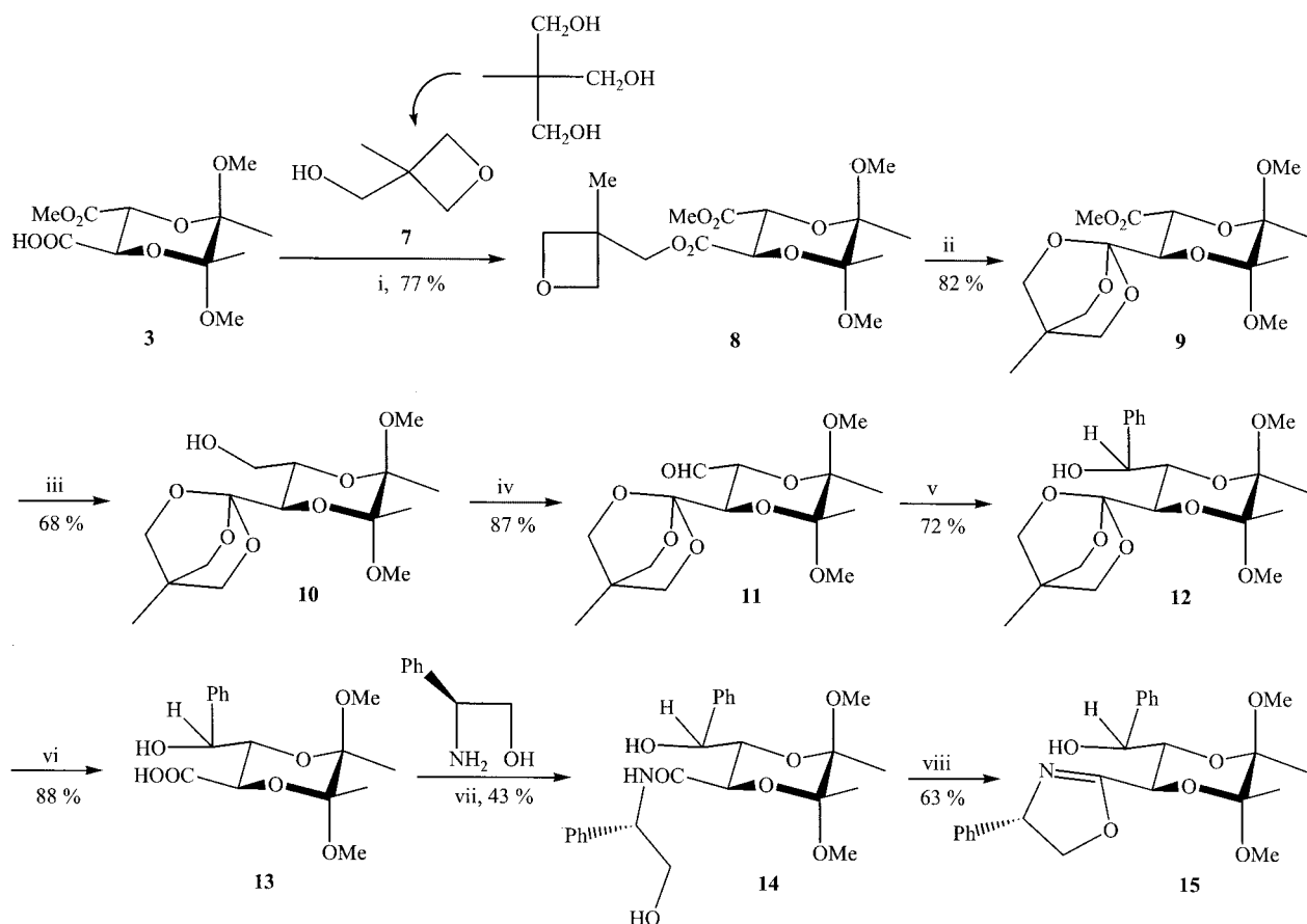
Scheme 2. Reagents and conditions: i) DCC, DMAP, \text{CH}_2\text{Cl}_2 , 0 °C, 4 h; ii) \text{BF}_3 \cdot \text{Et}_2\text{O} , \text{CH}_2\text{Cl}_2 , room temp., 1 h; iii) \text{LiAlH}_4 , THF, reflux; iv) (\text{COCl})_2 , DMSO, \text{Et}_3\text{N} , \text{CH}_2\text{Cl}_2 , -60 °C; v) \text{PhMgBr} , THF, reflux, 1 h 30; vi) 1 M HCl, pH 1, 0 °C, 40 min, then 1 M LiOH, pH 11, reflux; vii) amino alcohol, xylene, reflux, 17 h; viii) p\text{TsCl} , \text{Et}_3\text{N} , \text{CH}_2\text{Cl}_2 , reflux, 17 h
